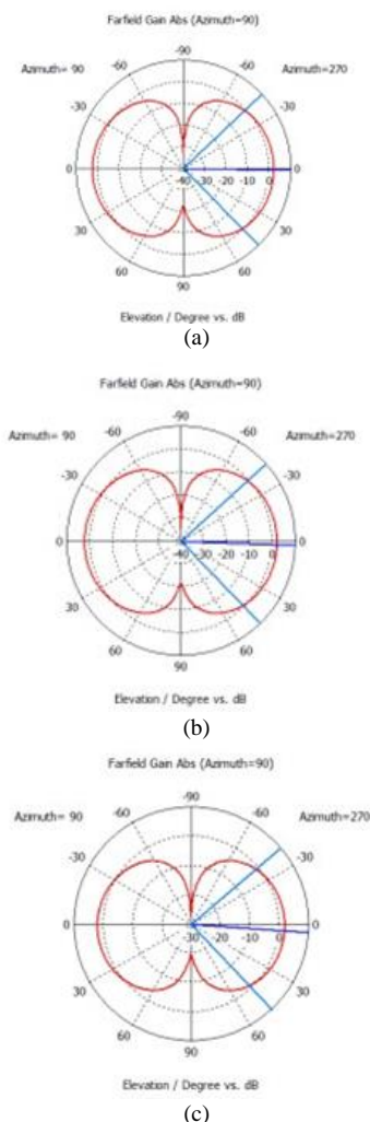
Figure 7: Radiation pattern at (a) 2.18GHz (b) 2.46GHz (c) 2.80GHz
