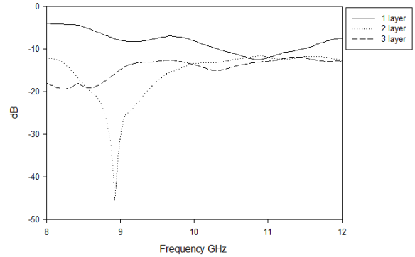
Figure 10: Absorption against frequency for plywood applied with palm ash
