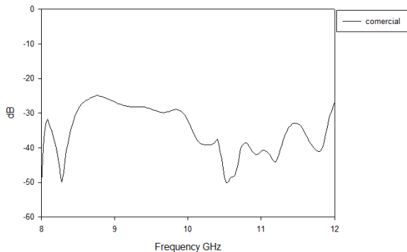
Figure 2: The ETS-Lindgren Rantec Flat Laminated Microwave Absorber performance
