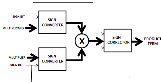
Figure 2: Multiplier Block
