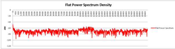
Figure 3: Flat Power Spectrum of the FPGA Channel Emulator
