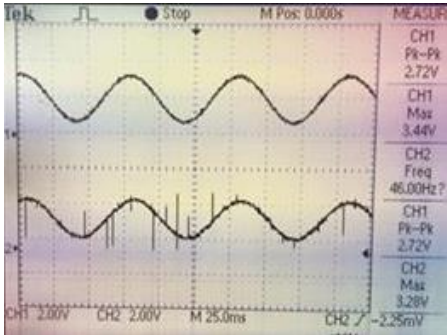
Figure 4: Input-Output Pair for 46 Hz Input sine wave at TF=1
