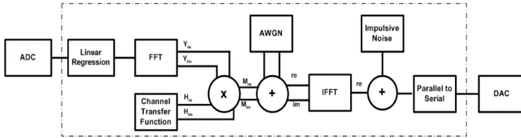
Figure 1: Block Diagram of the Narrowband PLC Channel Emulator
