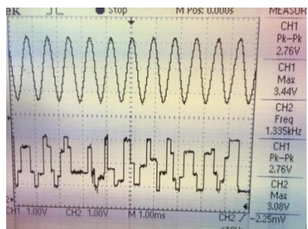
Figure 6: Input-Output Waveforms for 1.33-kHz Sine Input at TF=1
