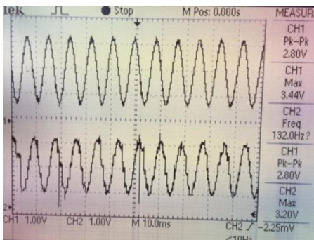
Figure 5: Input-Output Waveforms for 132 Hz Sine Input at TF=1
