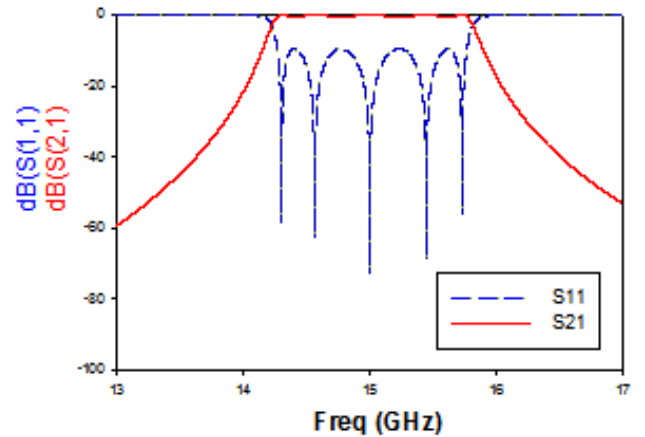
Figure 5: S21 and S11 of 15 GHz lumped-element bandpass filter
