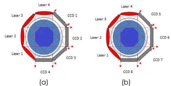
Figure 1 CCD and laser orientation for (a) upper plane and (b) lower plane
