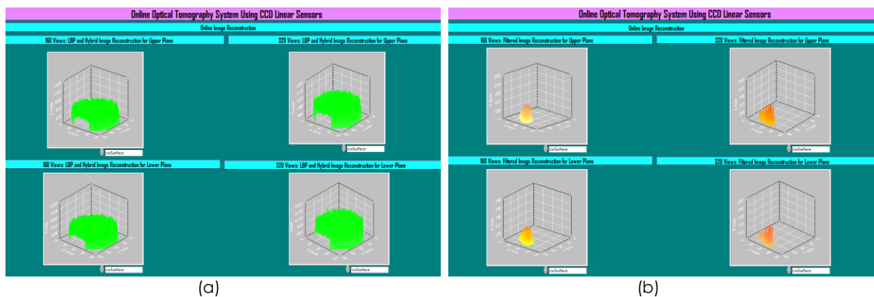
Figure 4 Labview front panel for optical tomography system using CCD sensor with (a) LBP with Hybrid and (b) filtered algorithms
