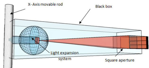
Figure 2 Laser diode expansion system box
