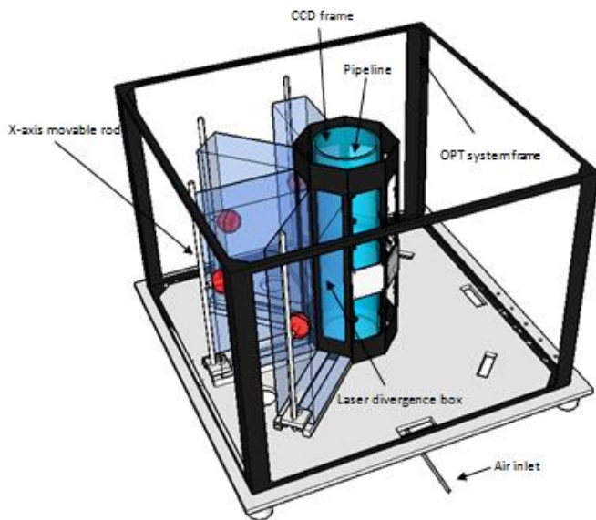
Figure 3 Hardware construction schematic diagram
