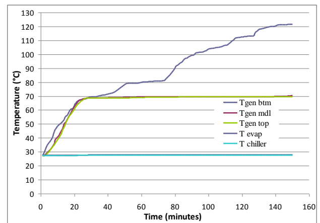
Figure 2 Adsorbent bed's temperature behaviour against desorption time
