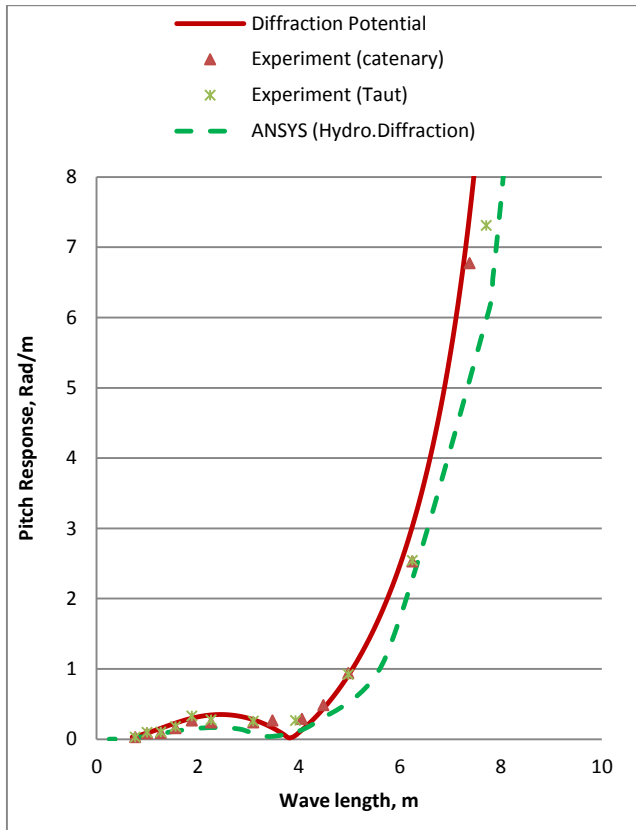
Figure 9 Pitch motion response of round shape FPSO
