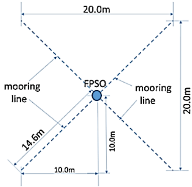
Figure 3 Arrangement of mooring lines and anchor basin
