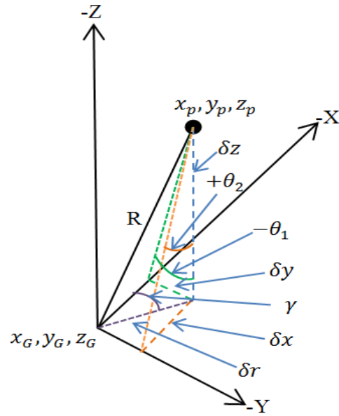
Figure 5 The relations between the positions of reflective optical tracking markers with position of center of gravity of model by consider the roll, pitch and yaw motions are showed in Figure 5.
