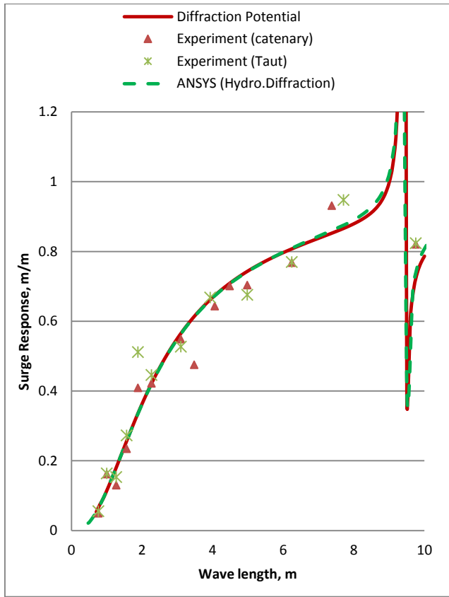
Figure 8 Surge motion response of round shape FPSO
