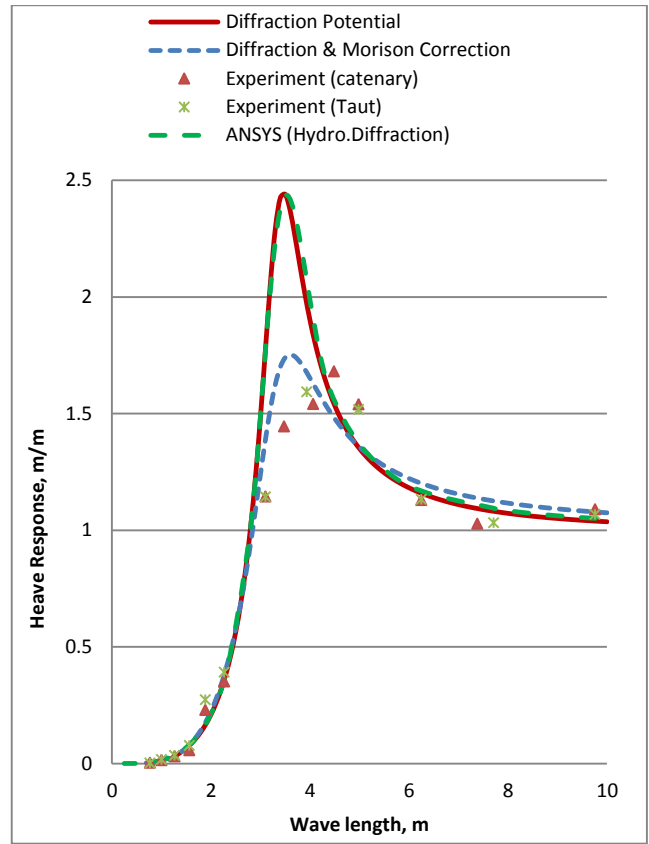
Figure 10 Heave motion response of round shape FPSO
