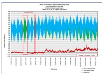
Figure 1. Differentiated graph for tidal observation and tidal prediction at Bayang Lagoon, Penang during El Niño effect
