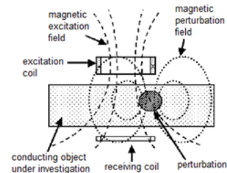
Figure 2 The principle of magnetic induction tomography [25]
