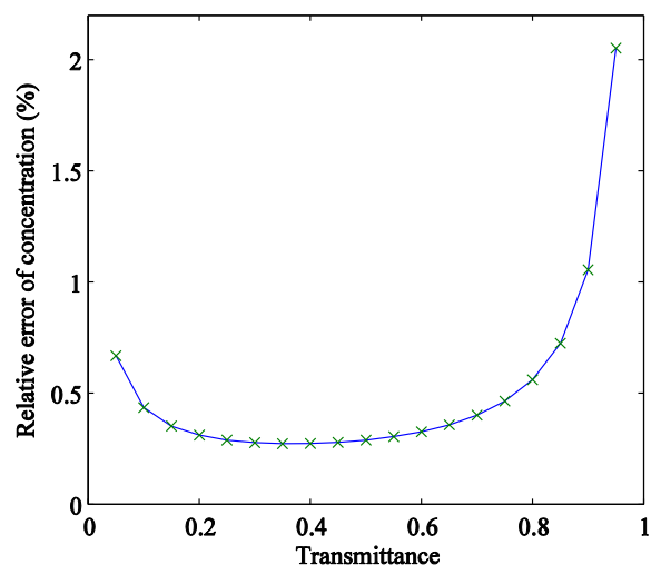
Figure 1 Twyman-Lothian curve based on absolute transmittance error 0.001
