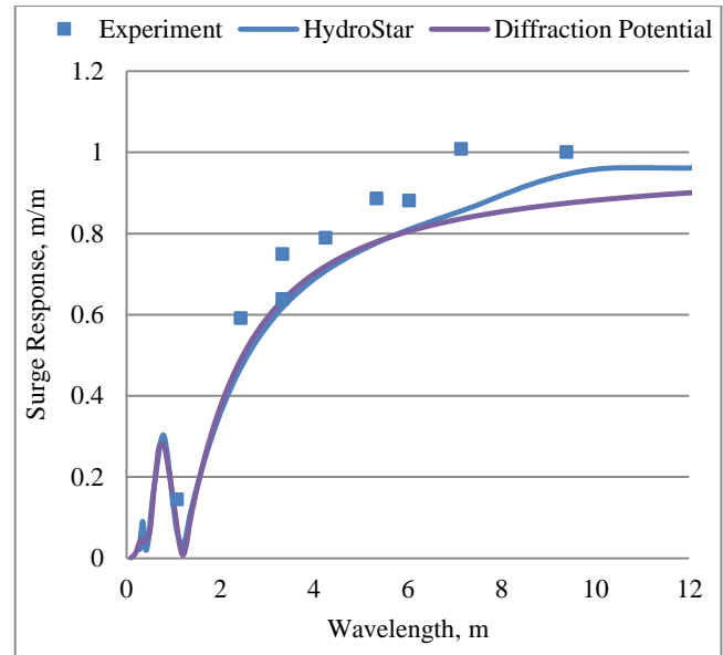
Figure 3 Surge motion response for semi-submersible model
