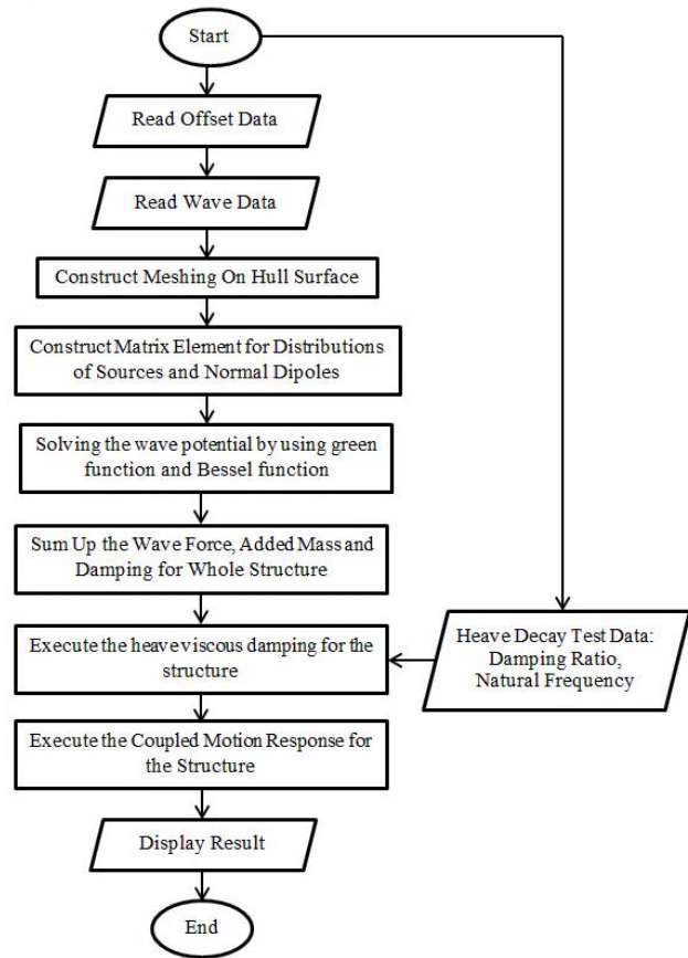
Figure 2 Flow chart for diffraction potential numerical method
