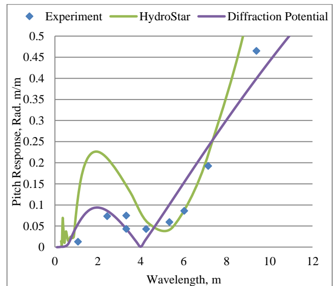
Figure 4 Pitch motion response for semi-submersible model
