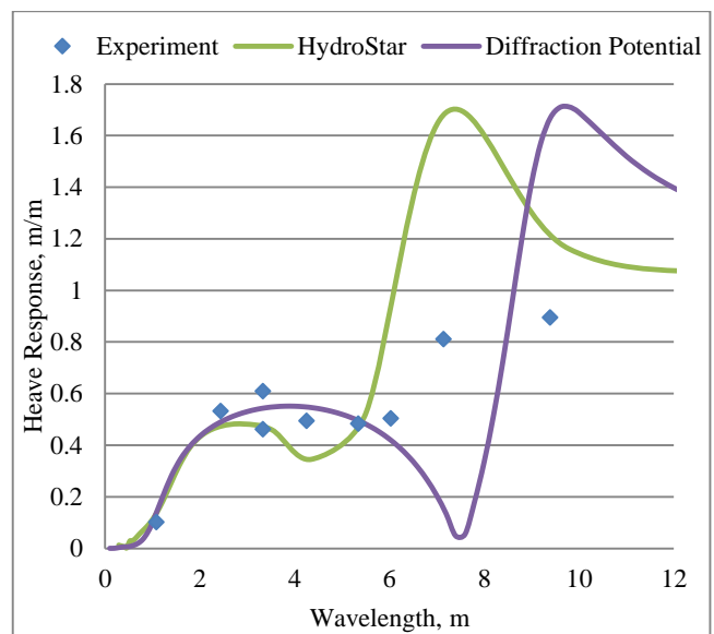
Figure 5 Heave motion response for semi-submersible model
