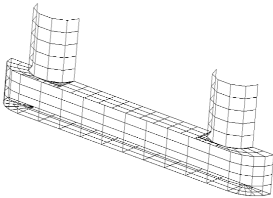
Figure 1 Meshing for semi-submersible model
