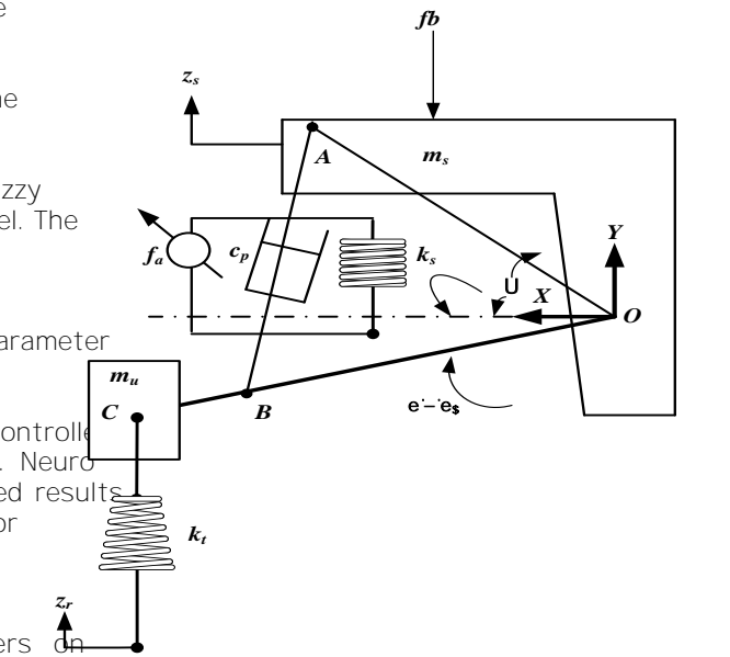
Figure 1 A free body diagram of a quarter car MacPherson strut model
