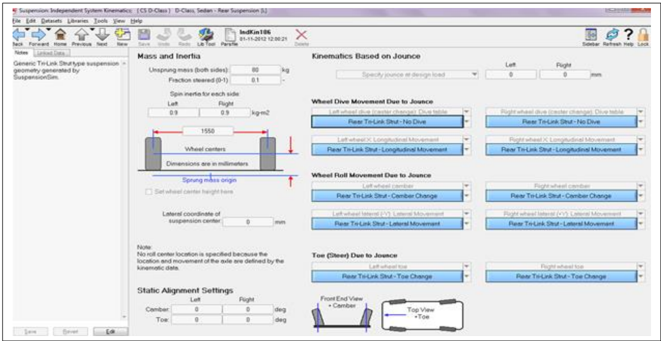
Figure 3 Control screen for active suspension parameter setup
